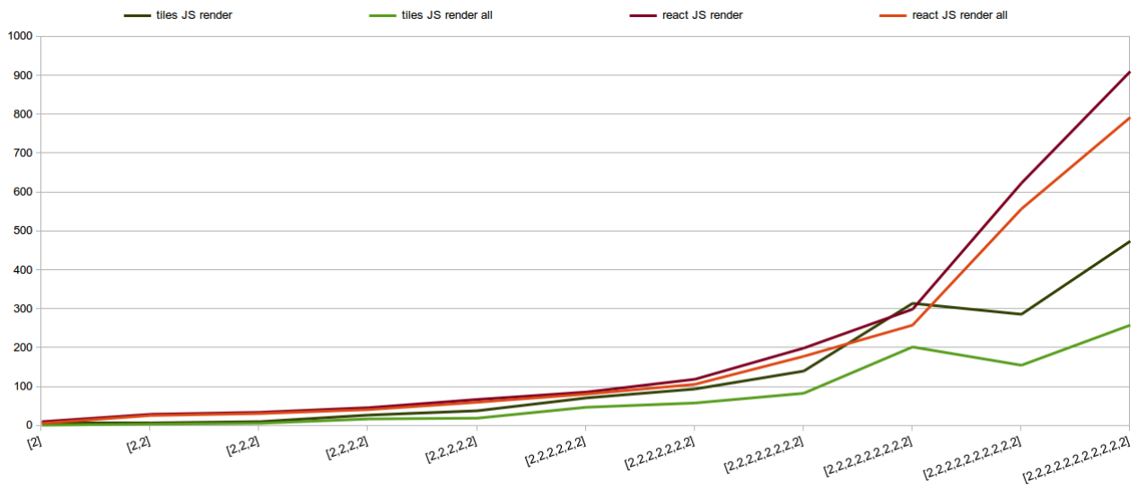
Figure 6.7: Comparison of the creation of the virtual DOM and rendering into the real DOM in the structure
