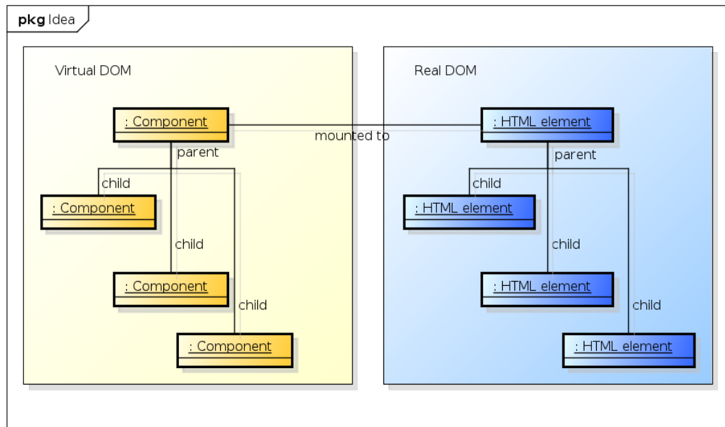
Figure 4.2: Virtual DOM
